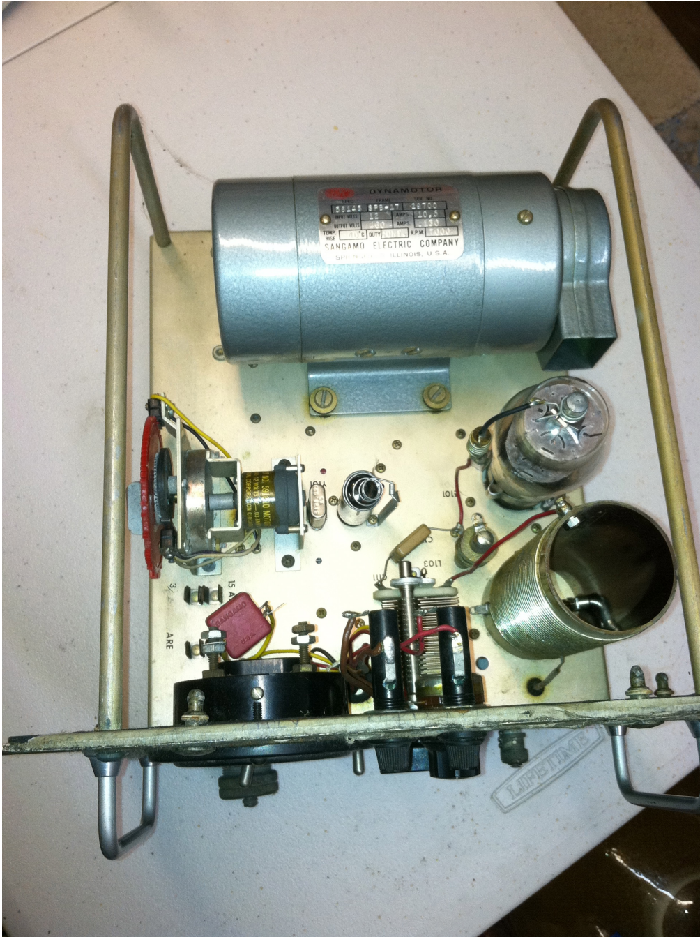
The transmitter and its dynamotor
